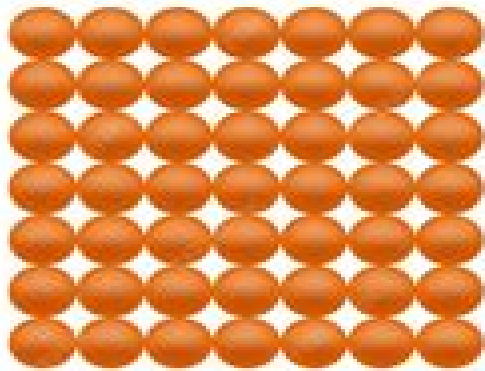
Low Entropy
